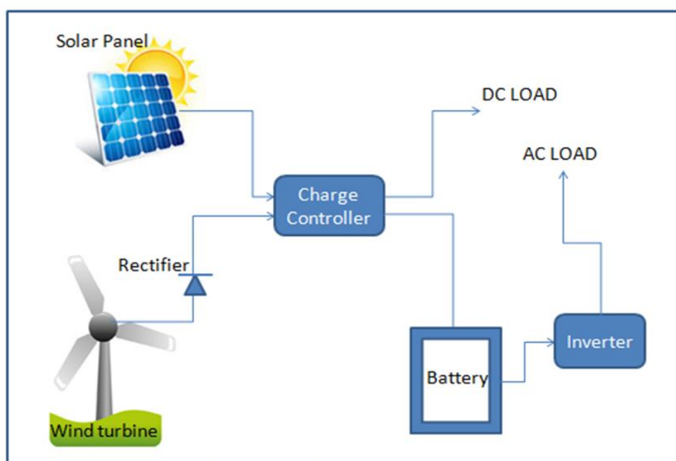
Fig 3. Hybrid Solar-Wind System
