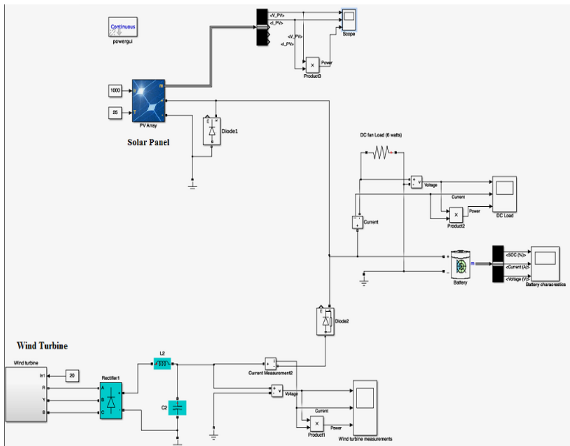
Fig 5. Circuit drawing of the Hybrid system in Simulink
