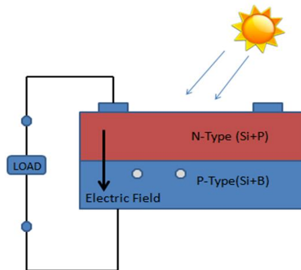
Fig 1. Solar Cell
