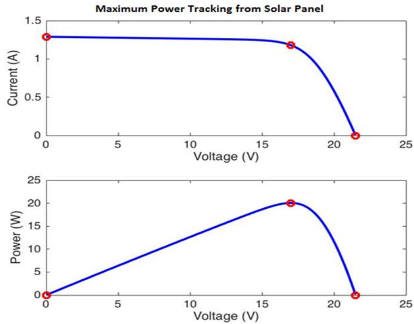
Fig 4. Simulation to find the Maximum Power from Solar Panel
